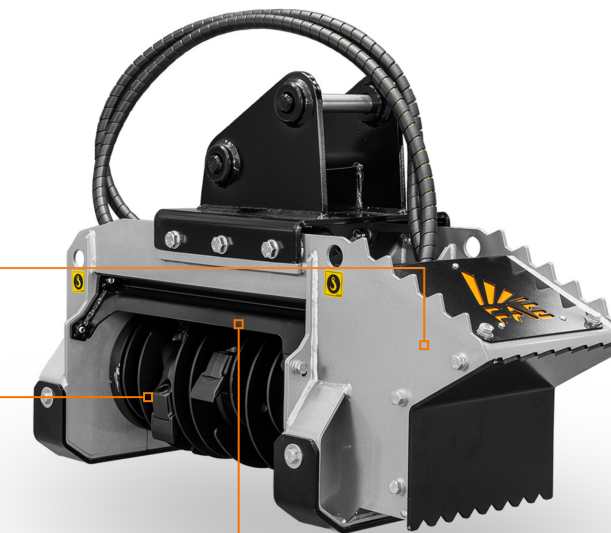
Fixed thumb bracket built into the frame useful for moving materials that need to be mulched
